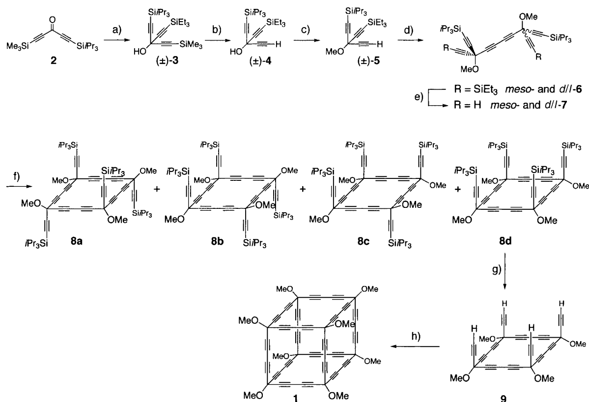
Scheme 2. Synthesis of the expanded cubane 1 . Reagents and conditions: a) \text{Et}_3\text{SiC}\equiv\text{CH} , BuLi, THF, 0^\circ\text{C} , 3 h, 95 %; b) 1N NaOH, MeOH/THF (1/1), RT, 1 h, 86 %; c) BuLi, THF, -78^\circ\text{C} , 10 min, then MeI, -78^\circ\text{C}\rightarrow\text{RT} , 16 h, 98 %; d) CuCl, TMEDA, air, \text{CH}_2\text{Cl}_2 , RT, 5 h, 97 %; e) \text{K}_2\text{CO}_3 , MeOH/THF (1/1), RT, 2.5 h, 93 %; f) CuCl, TMEDA, air, \text{CH}_2\text{Cl}_2 , RT, 18 h, 8 % ( 8a ), 18 % ( 8b ), 36 % ( 8c ), 10 % ( 8d ); g) \text{Bu}_4\text{NF} , wet THF, -15^\circ\text{C} , 2.5 h, 87 %; h) CuCl, TMEDA, air, \text{CH}_2\text{Cl}_2 , RT, 3 h, 16 %. TMEDA = N,N,N',N' -tetramethyl-1,2-ethanediamine.
